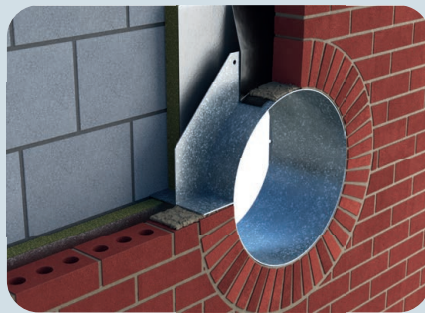
Bull's Eye Lintel
